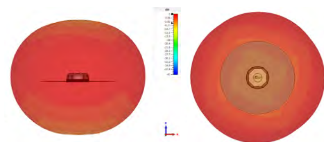
Radiation Patterns at 850 MHz
