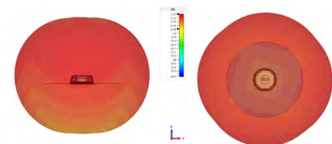
Radiation Patterns at 1500 MHz
