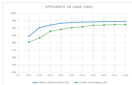
Figure 5. Efficiency Curves at 28V Output Voltage
