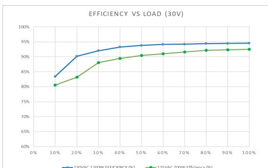
Figure 6. Efficiency Curves at 30V Output Voltage
