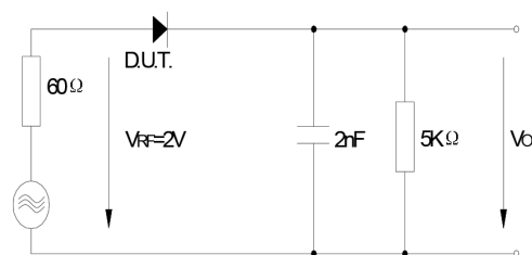
FIG.4 – RECTIFICATION EFFICIENCY MEASUREMENT CIRCUIT
