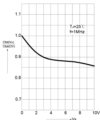
FIG.5 – RELATIVE CAPACITANCE VERSUS VOLTAGE
