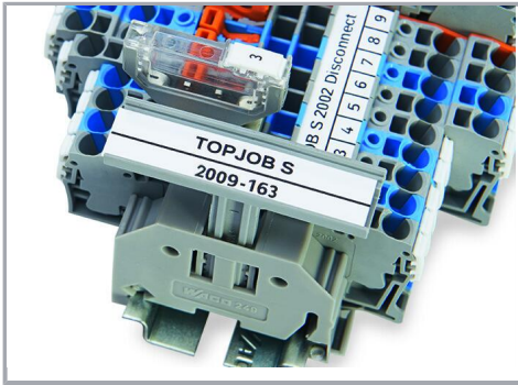
Height-adjustable group marker carrier (2009-163) for WMB markers or marking strips (2009-110)
