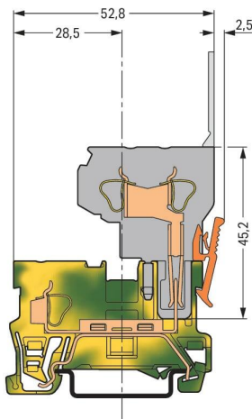
Ground carrier terminal block
