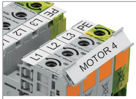
Marker carrier (285-442) for marking strips (2009-110) or 2 WMB markers for 285-13x, 285-15x and 285-19x Terminal Blocks
