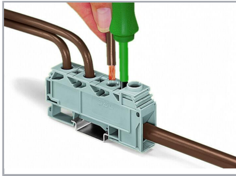
Terminating a 10 mm 2 (8 AWG) conductor –
