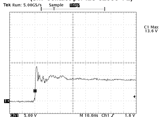
ESD Clamping
