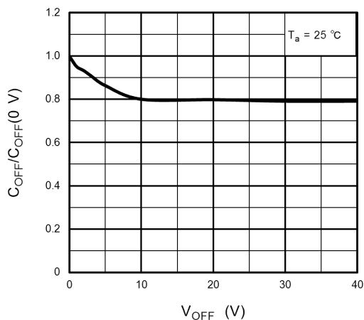
Fig. 12.1.11 C_{OFF}/C_{OFF(0V)} - V_{OFF}
