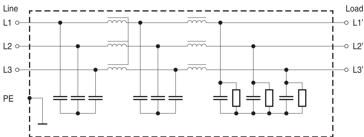
B84143K*S081
