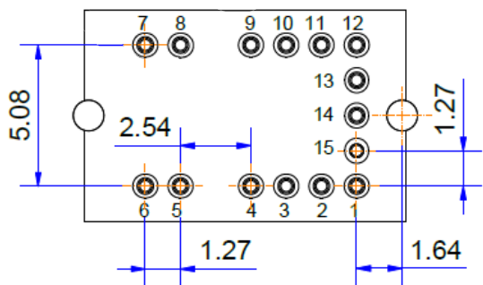
Figure 2: Module Bottom View (Dimensions in mm)
