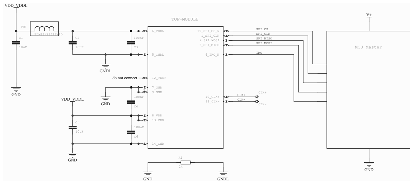
Figure 23: Application Schematic
