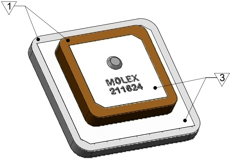
3D VIEW
