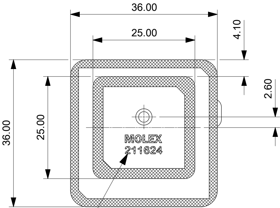
INK MARK
