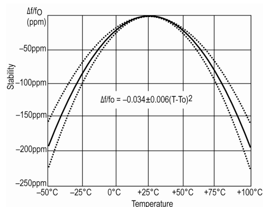
Typical Frequency Stability Characteristics
