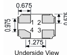
Underside View
