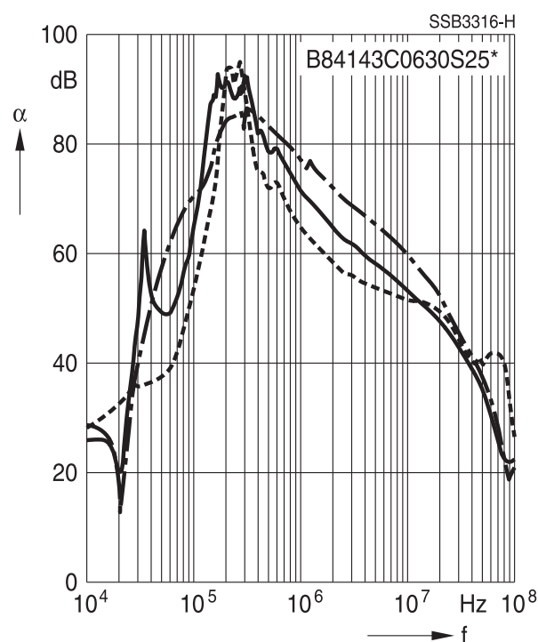
Filters for 630 A
