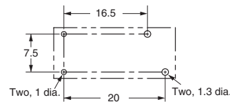
PCB Mounting Holes (Bottom View) Tolerance: \pm 0.1 mm
