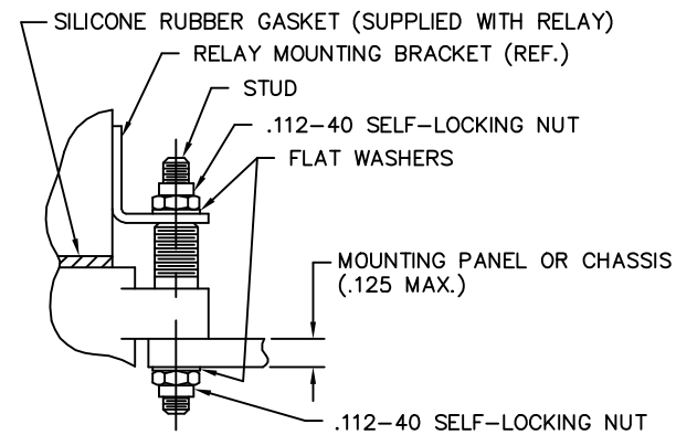
TOP MOUNT
