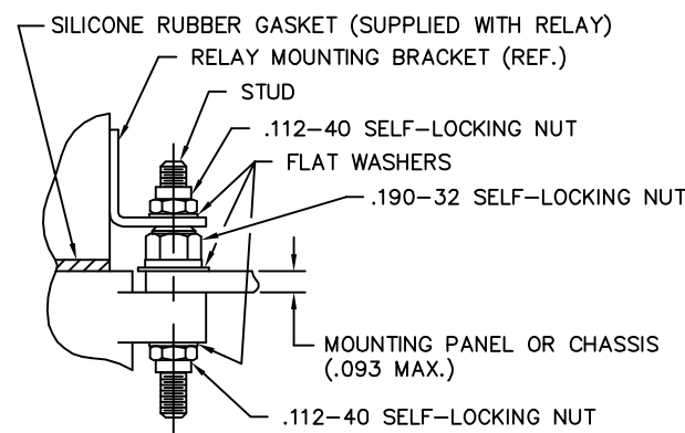
BOTTOM MOUNT
