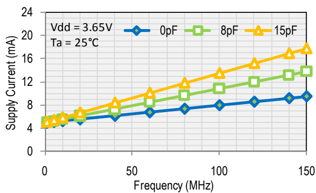
Supply Current
