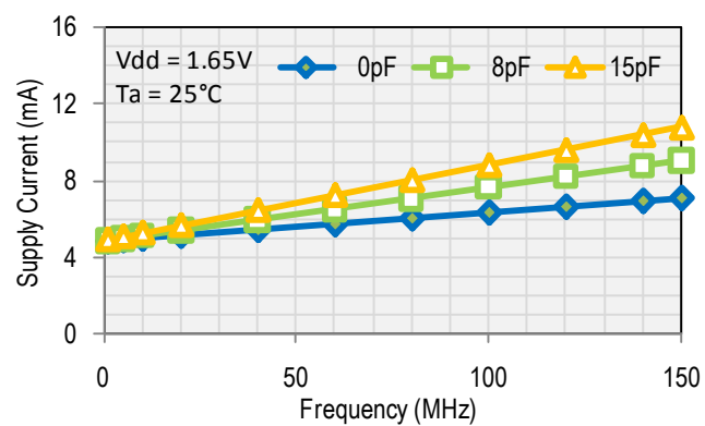
Supply Current
