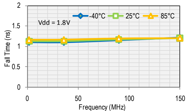
Fall Time
