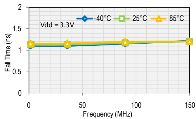
Fall Time
