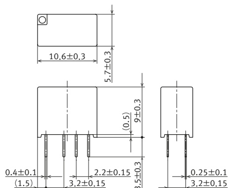
External dimensions
