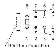
Schematic ( TOP VIEW ) Single side stable High sensitivity single side stable ( De-energize )
