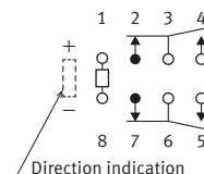
Schematic ( BOTTOM VIEW ) Single side stable High sensitivity single side stable ( De-energize )
