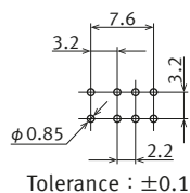
Recommended PC board pattern (BOTTOM VIEW)
