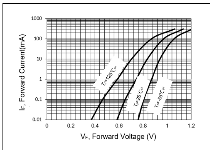
Figure 4. Forward Characteristics Curve
