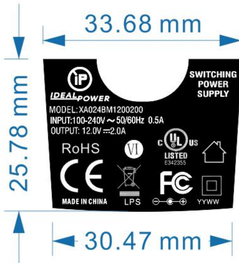
Nameplate
