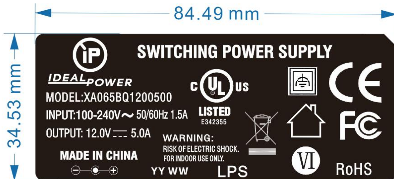
Nameplate
