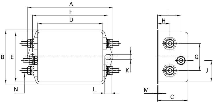
Connection style -08, 16 and 20 A types
