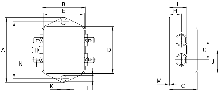
Connection style -06, 1 to 12 A types
