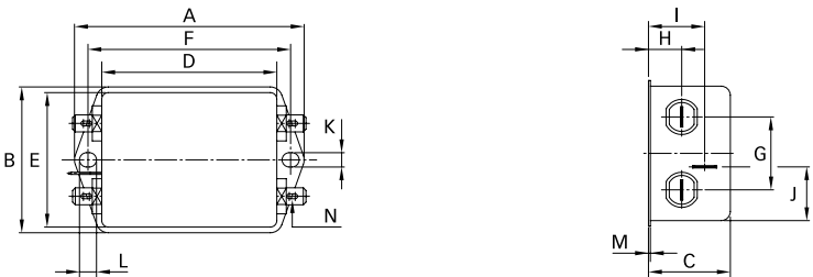
Connection style -06, 16 and 20 A types
