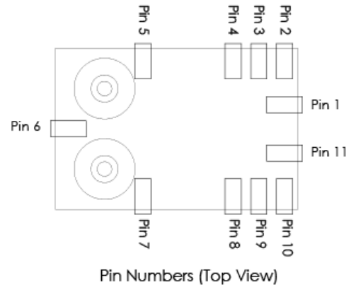
SM02 Package Pinout
