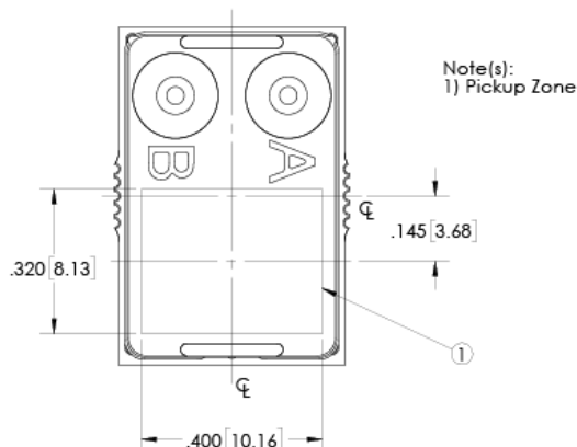
SM02 Pick and Place Pickup Zone
