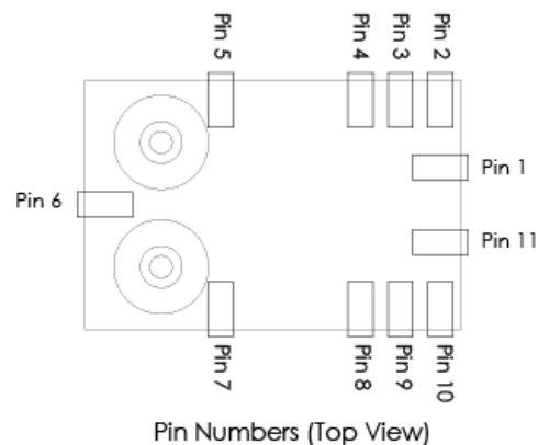
SM02 Package Pinout
