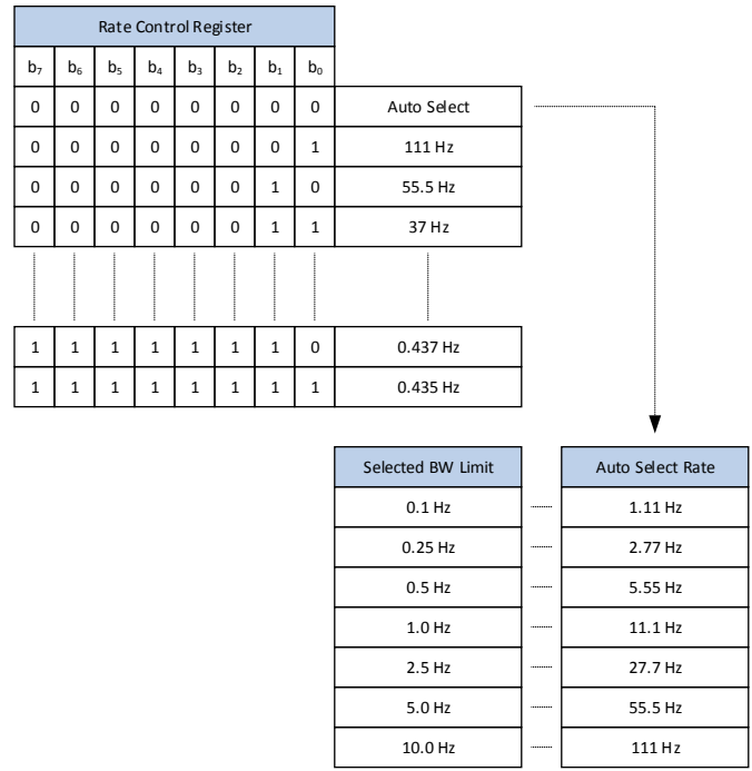
Rate Control Register Detail
