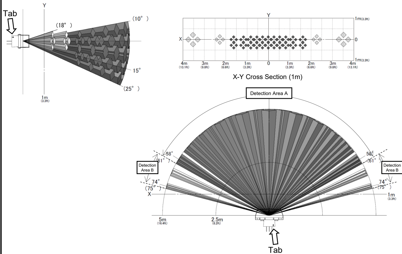
Side View
