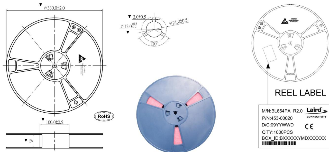
Figure 14: Reel specifications
