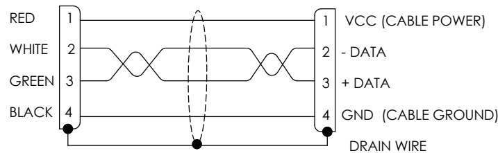
"P1" WIRING DIAGRAM "J1"
