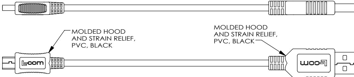
"P1" SERIES "B" MINI 5 PIN PLUG CONTACTS: 30 \mu INCHES GOLD PLATING
