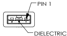
"P2" USB SERIES "A" PLUG CONTACTS: 30 \mu INCHES GOLD PLATING
