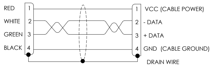
WIRING DIAGRAM
