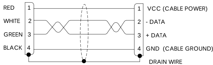
"P1" WIRING DIAGRAM
