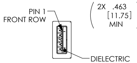
"P1" USB 3.0 SERIES "A" PLUG CONTACTS 30μ GOLD
