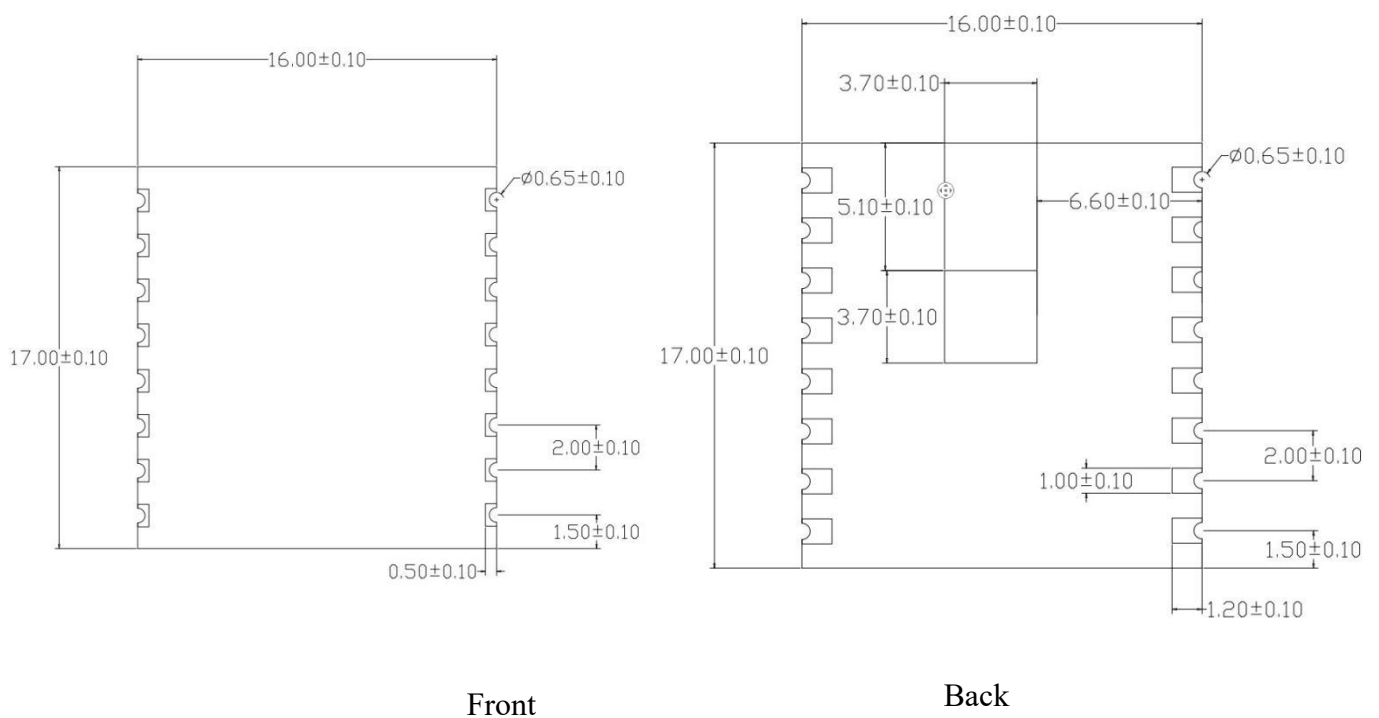
Figure 4 Dimension diagram(unit:mm)
