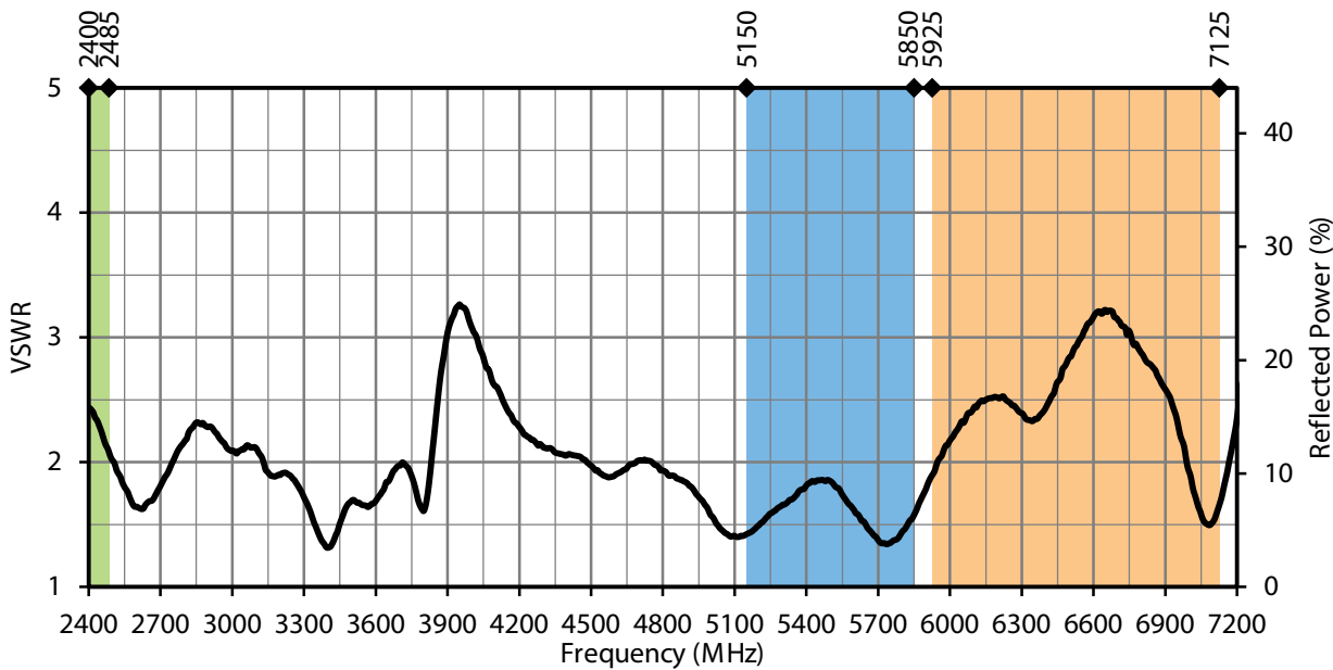
Figure 11. W63WS3 VSWR, Edge-Bent
