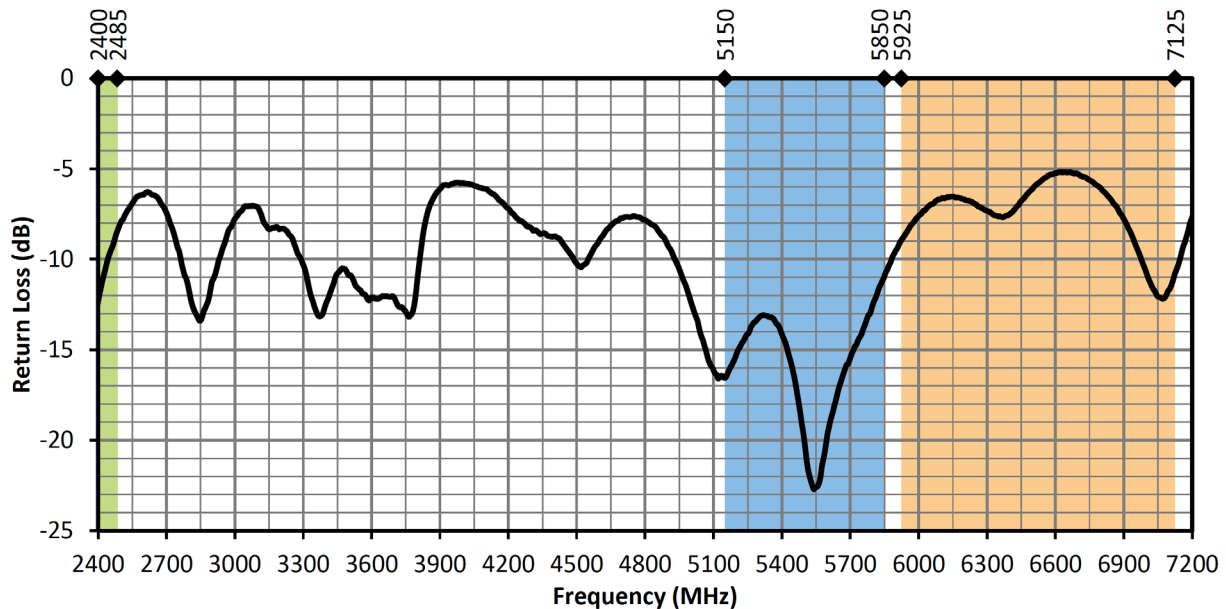
Figure 4. W63WS3 VSWR, Straight
