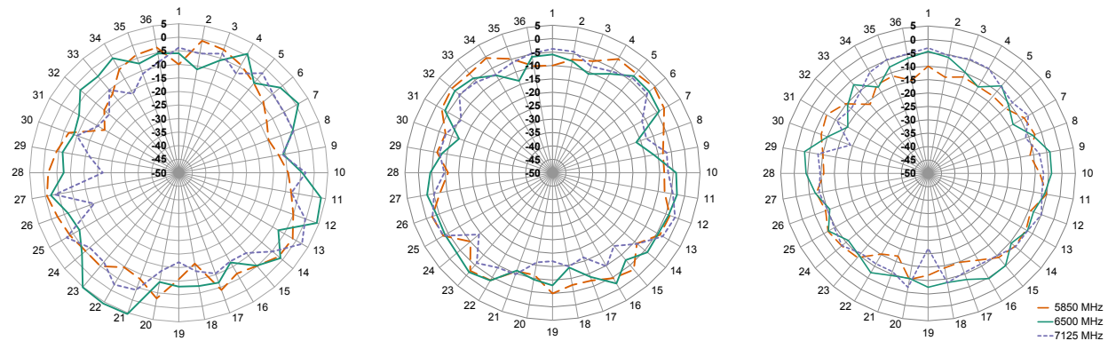
Figure 16. Radiation Patterns for ANT-W63WS3-SMA, Edge-Bent
