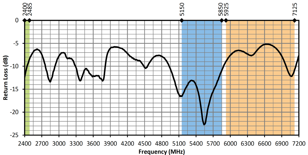
Figure 5. W63WS3 Return Loss, Straight
