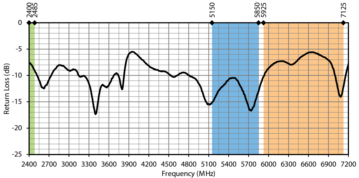
Figure 12. W63WS3 Return Loss, Edge-Bent
