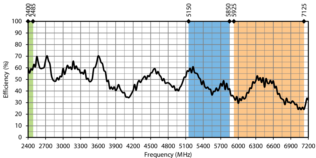
Figure 15. W63WS3 Antenna Efficiency, Edge-Bent
