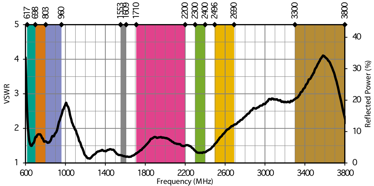
Figure 2. RPC Antenna VSWR with Frequency Band Highlights
