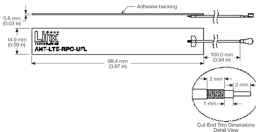
Figure 1. ANT-LTE-RPC-ccc Product Dimensions
