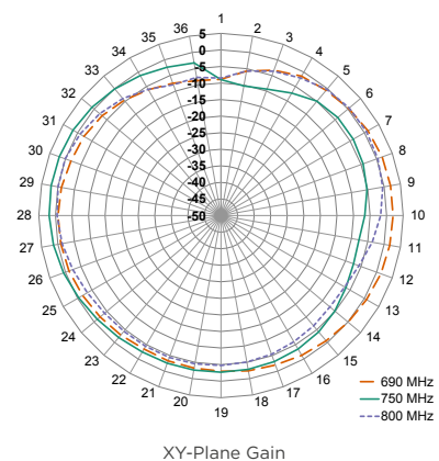
XY-Plane Gain
