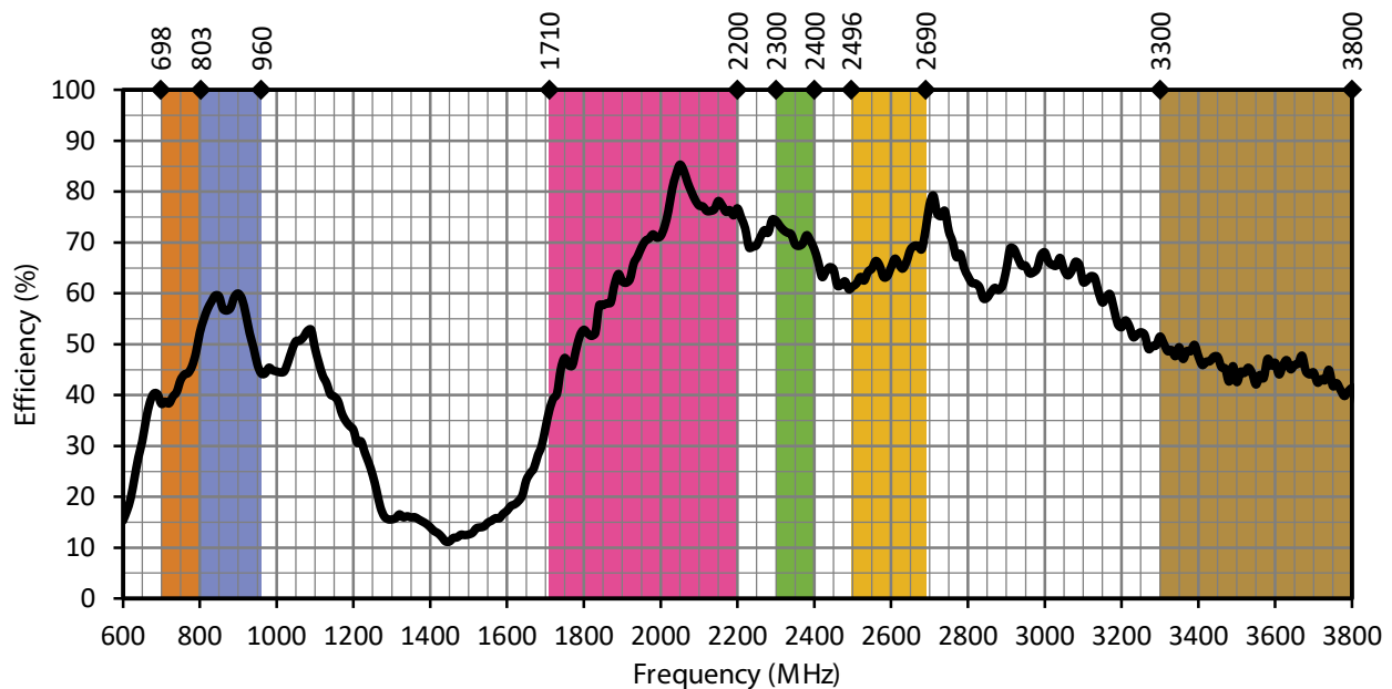
Figure 5. LPL Antenna Radiation Efficiency with Frequency Band Highlights
