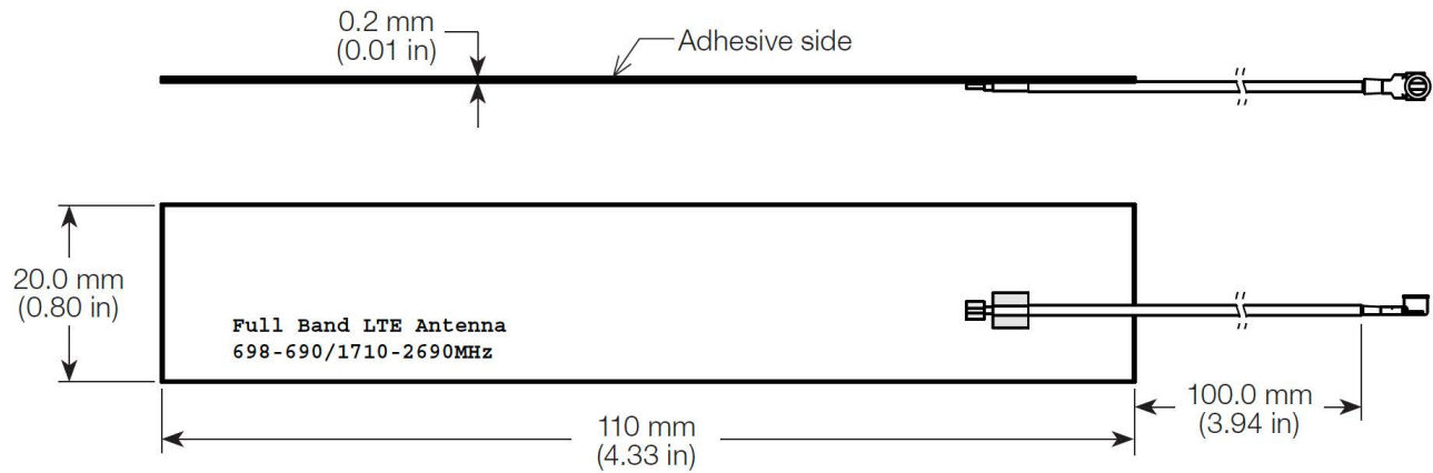
Figure 6. ANT-LPL-FPC-100 Dimensions
