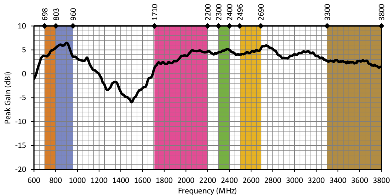
Figure 3. LPL Antenna Peak Gain with Frequency Band Highlights
