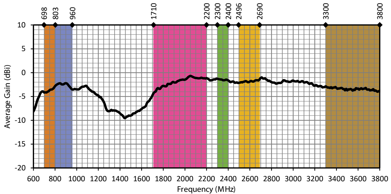
Figure 4. LPL Antenna Average Gain with Frequency Band Highlights
