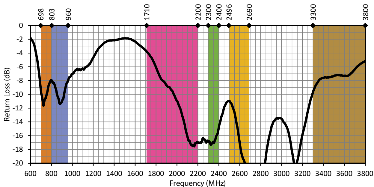
Figure 2. LPL Antenna Return Loss with Frequency Band Highlights
