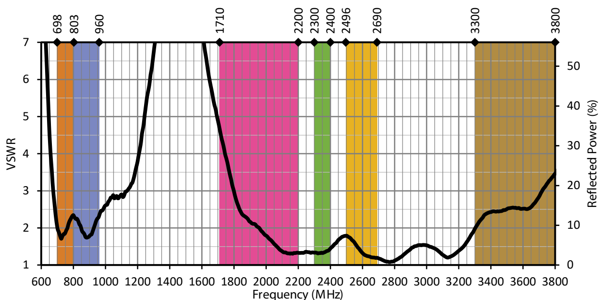
Figure 1: LPL Antenna VSWR with Frequency Band Highlights
