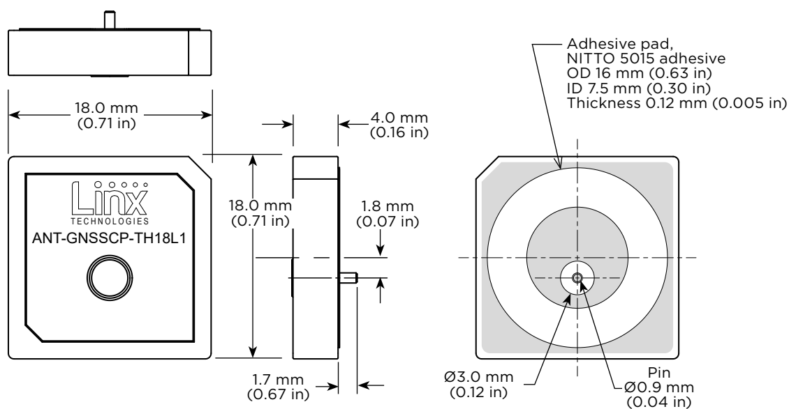
Figure 1. GNSSCP-TH18L1 Antenna Dimensions
