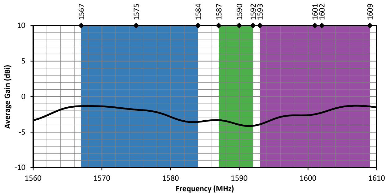
Figure 5. GNSSCP-TH18L1 Antenna Average Gain
