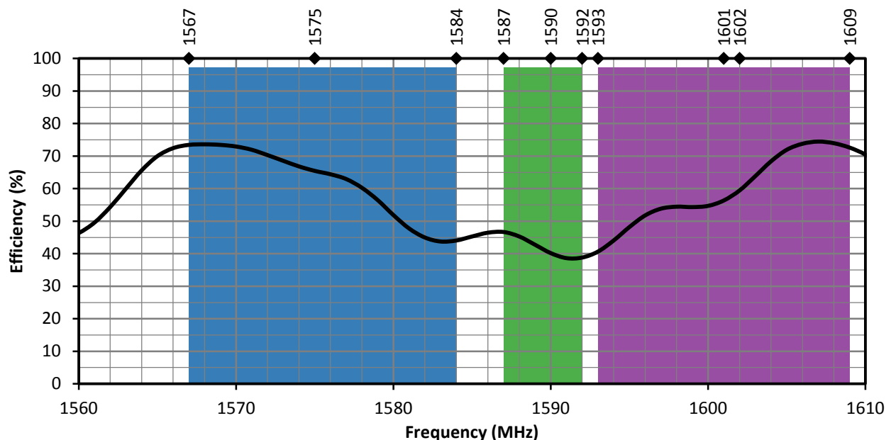
Figure 7. GNSSCP-TH18L1 Antenna Radiation Efficiency
