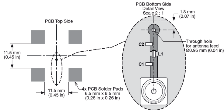
Figure 11. ANT-GNSSCP-TH18L1 Antenna Placement on PCB
