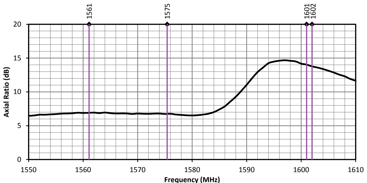
Figure 5. ANT-GNCP-C106L160 Antenna Axial Ratio
