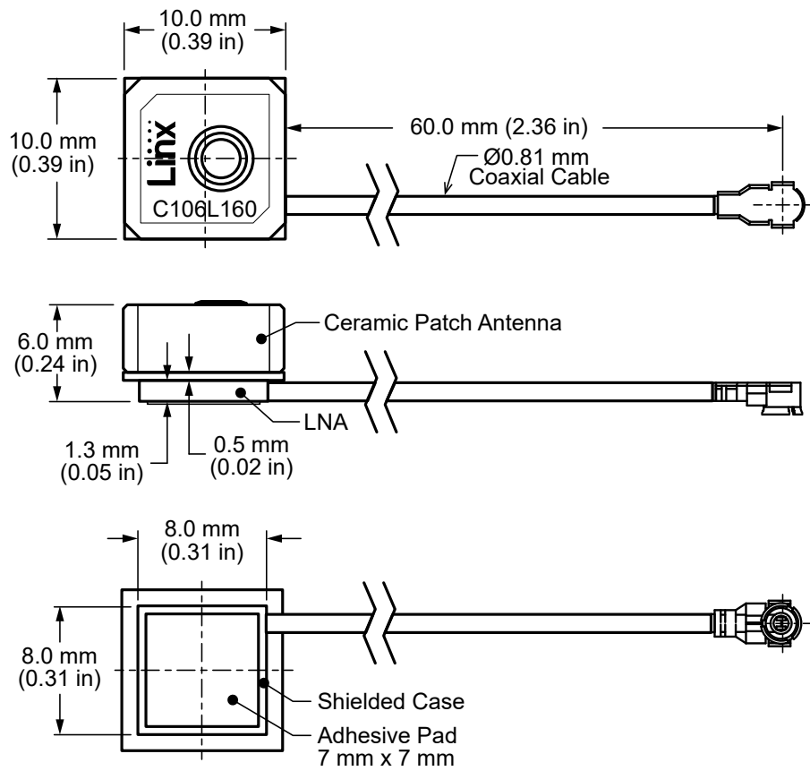
Figure 1. ANT-GNCP-C106L160 Antenna Dimensions
