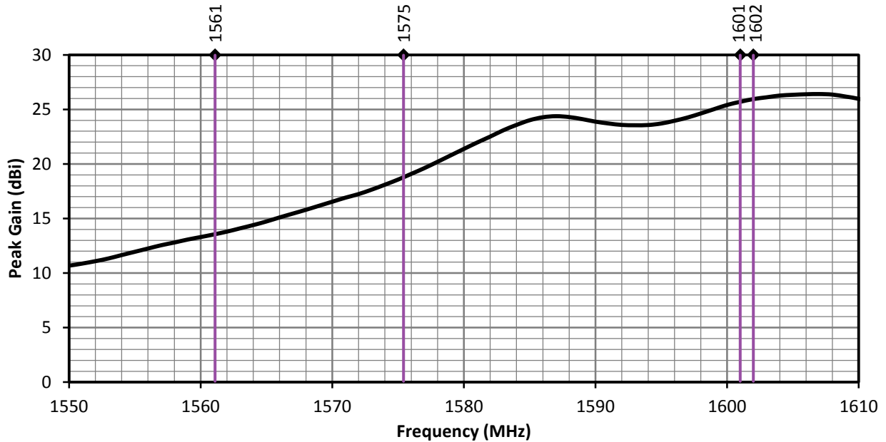
Figure 4. ANT-GNCP-C106L160 Peak Gain
