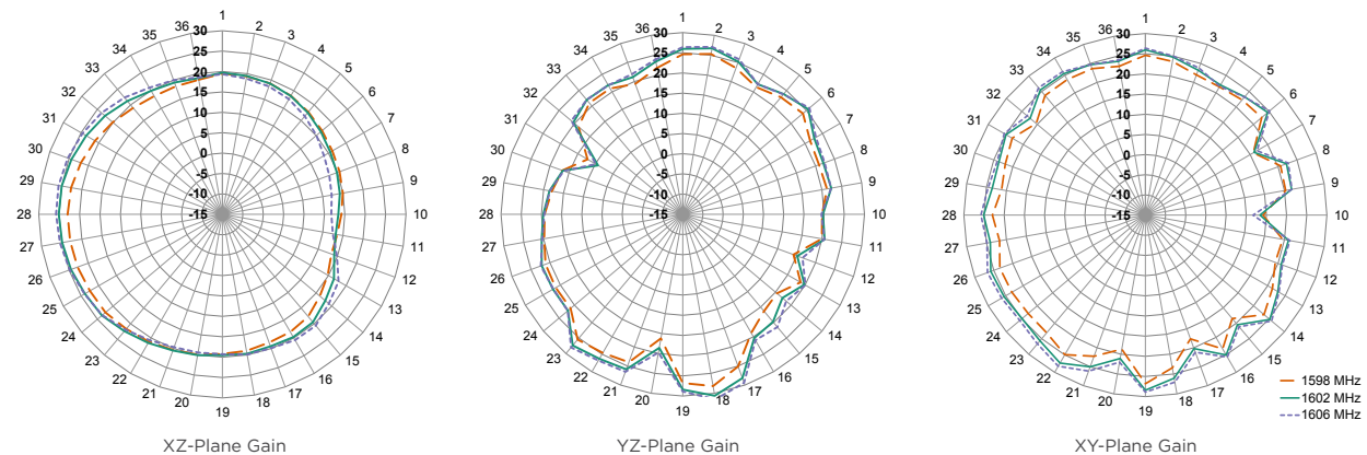
Figure 6. ANT-GNCP-C106L160 Radiation Patterns
