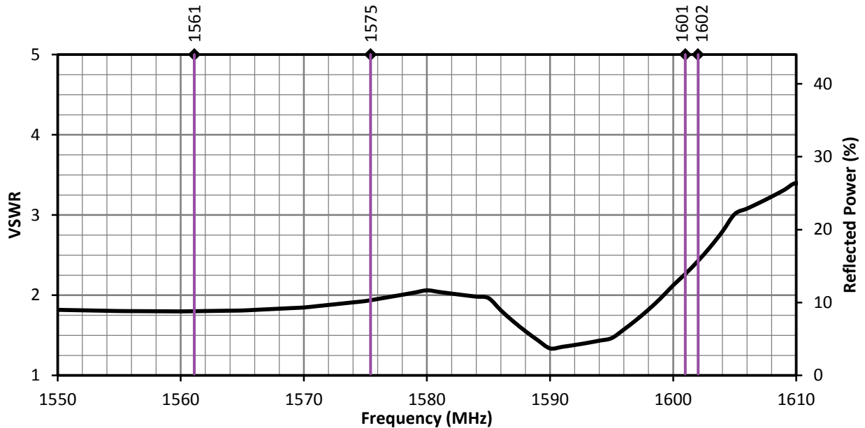
Figure 2. ANT-GNCP-C106L160 VSWR
