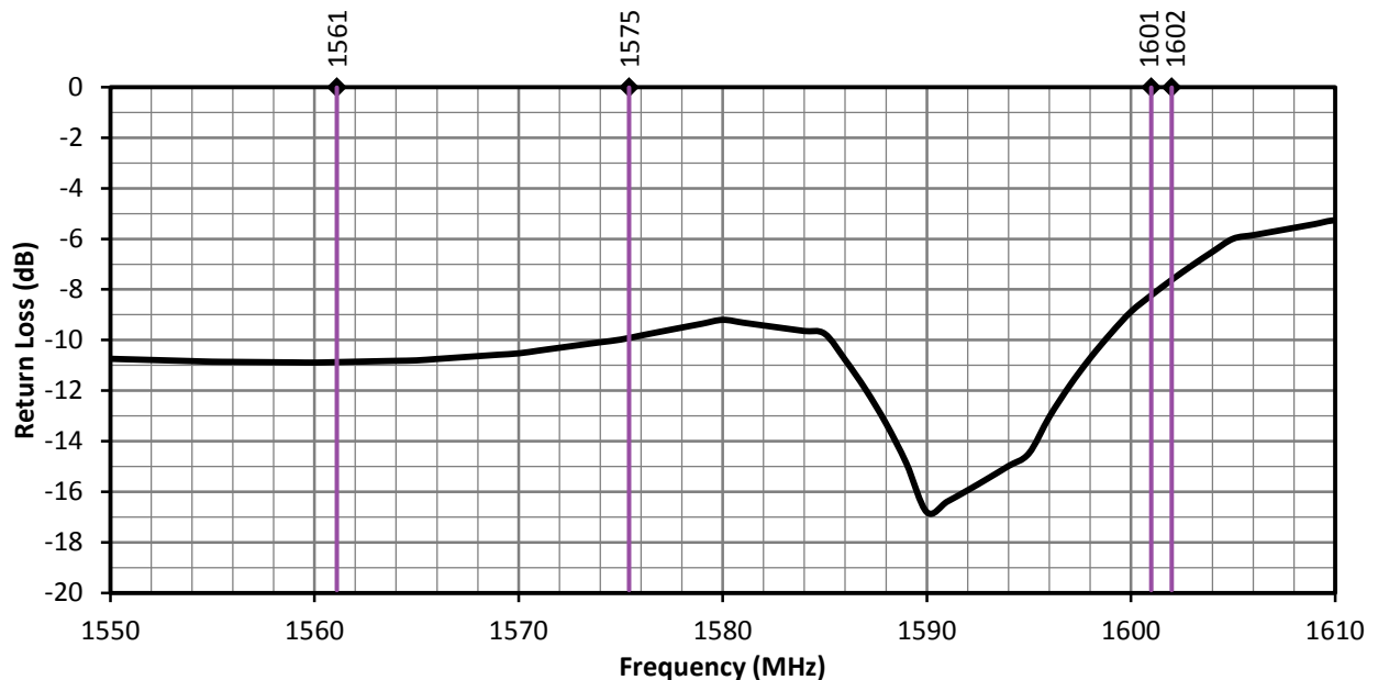
Figure 3. ANT-GNCP-C106L160 Return Loss
