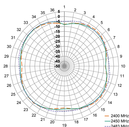
XY-Plane Gain
