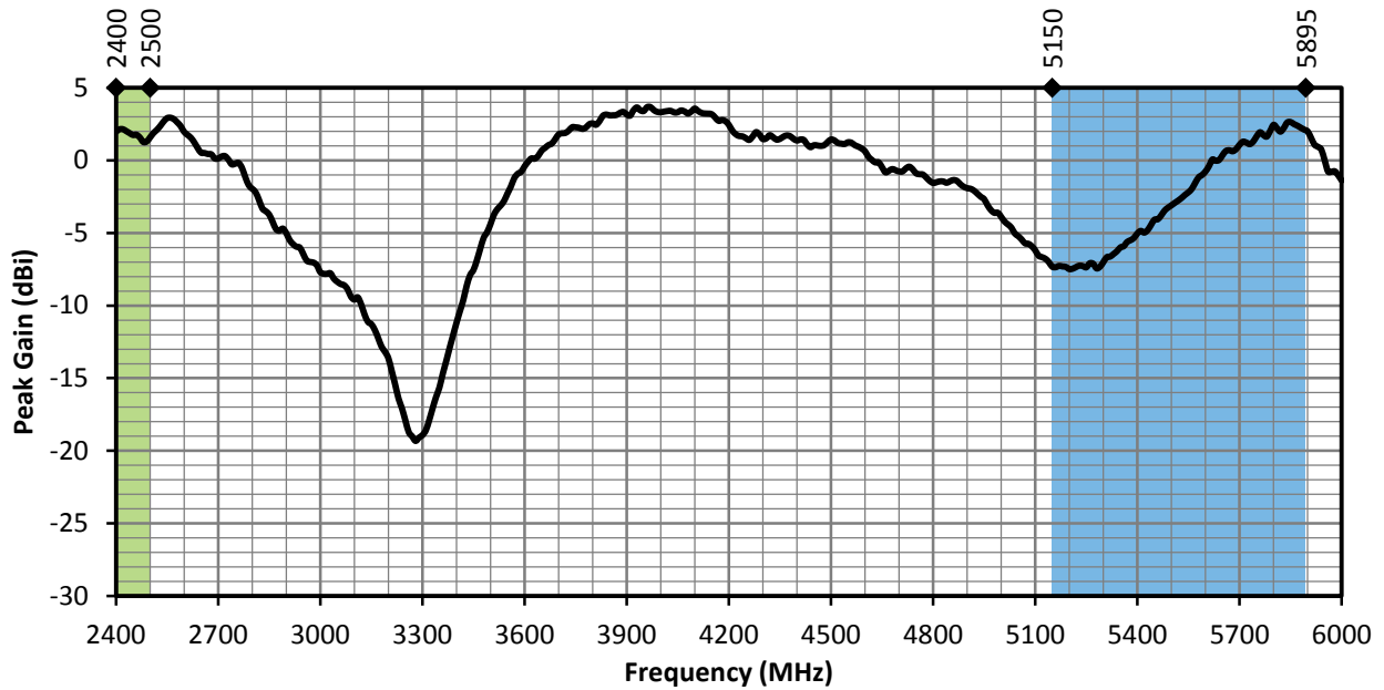
Figure 6. ANT-DB1-WRT-MON Peak Gain, with Frequency Band Highlights
