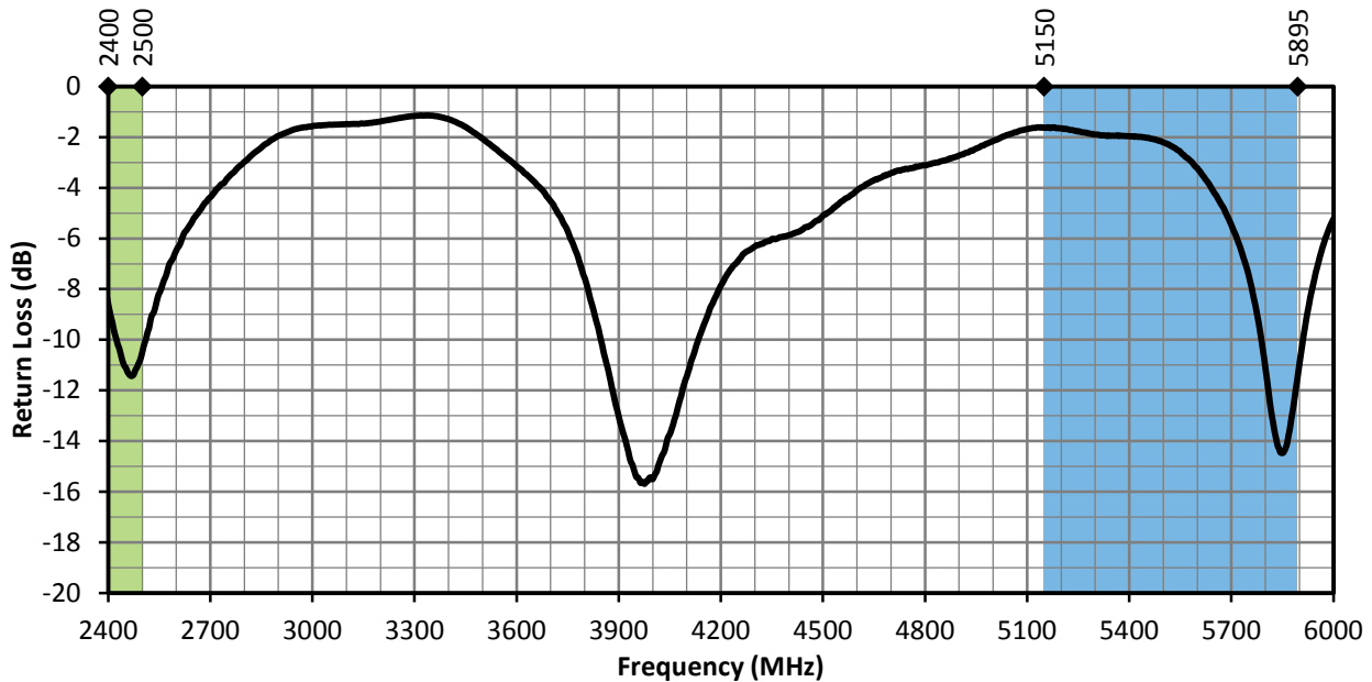
Figure 5. ANT-DB1-WRT-MON Return Loss, with Frequency Band Highlights
