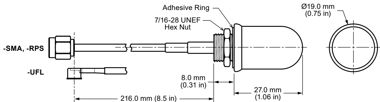
Figure 1. ANT-DB1-WRT-MON Antenna Dimensions
