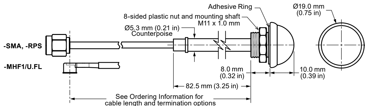
Figure 1. ANT-916-WRT Antenna Dimensions
