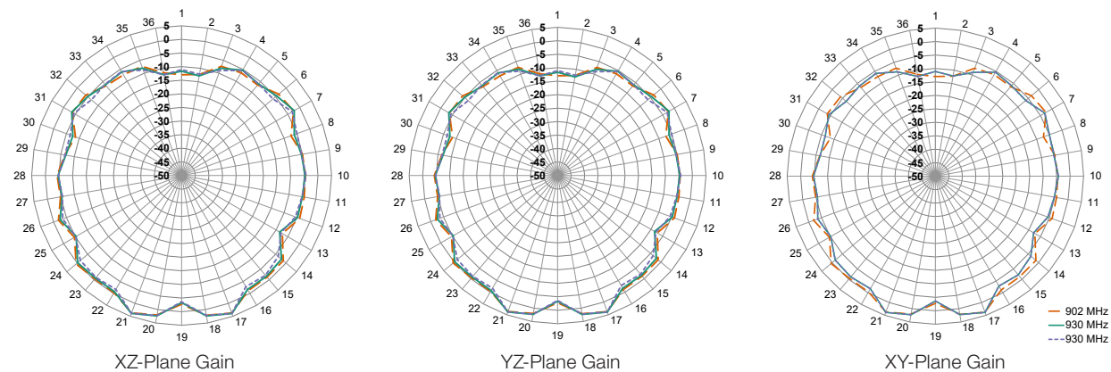
Figure 17. ANT-916-WRT Radiation Patterns, Center of Ground Plane
