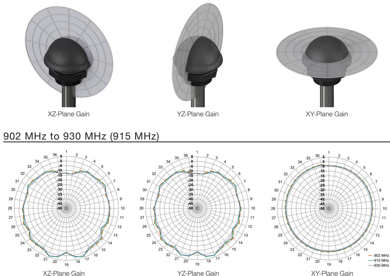
Figure 10. ANT-916-WRT Radiation Patterns, Free Space
