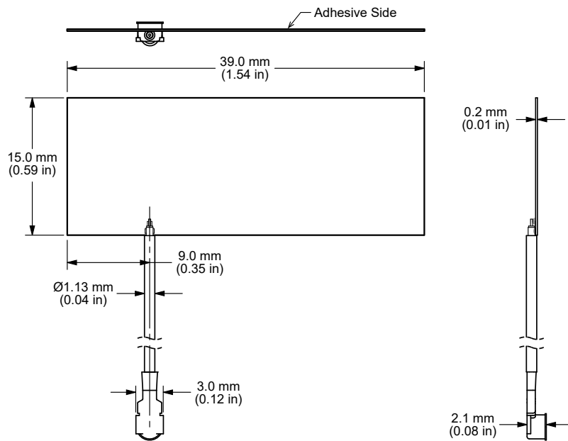
Figure 1: ANT-8/9-FPC-UFL Dimensions
