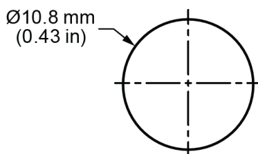
Figure 2. ANT-2.4-WRT Series Antenna Recommended Enclosure Mounting Dimensions
