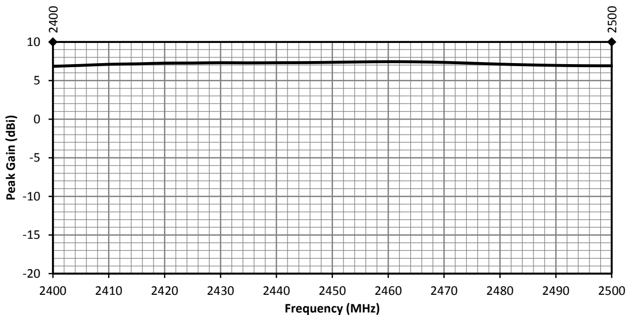
Figure 14. AANT-2.4-WRT Peak Gain at Center of Ground Plane
