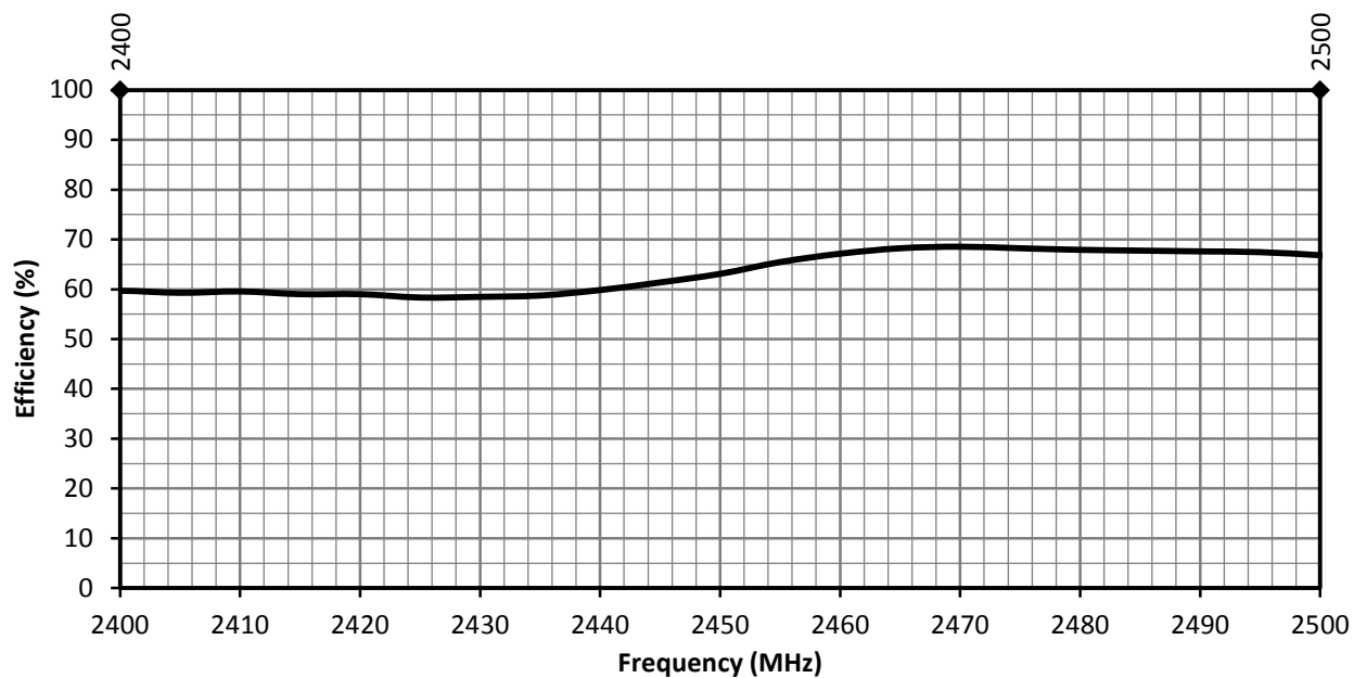
Figure 9. ANT-2.4-WRT Series Antenna Radiation Efficiency, Free Space
