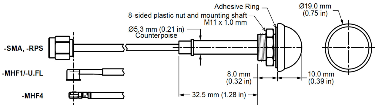
Figure 1. ANT-2.4-WRT Series Antenna Dimensions
