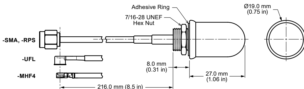
Figure 1: ANT-2.4-WRT-MON Antenna Dimensions
