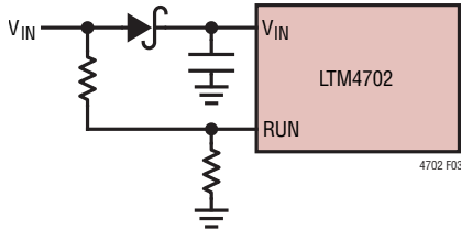
Figure 3. Reverse Input Protection
