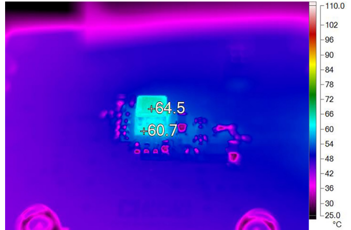
Figure 5. Thermal Image at 12V IN , 1V, 8A Output without Airflow and Heat Sink
