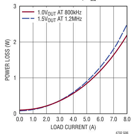
Power Loss vs Load, V_{IN} = 3.3\text{V}
