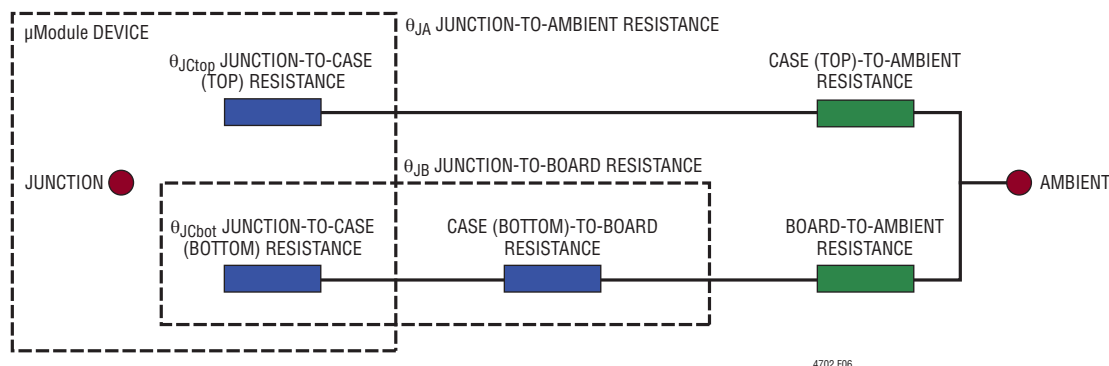
Figure 6. Graphical Representation of Thermal Coefficients, Including JESD51-12 Terms
