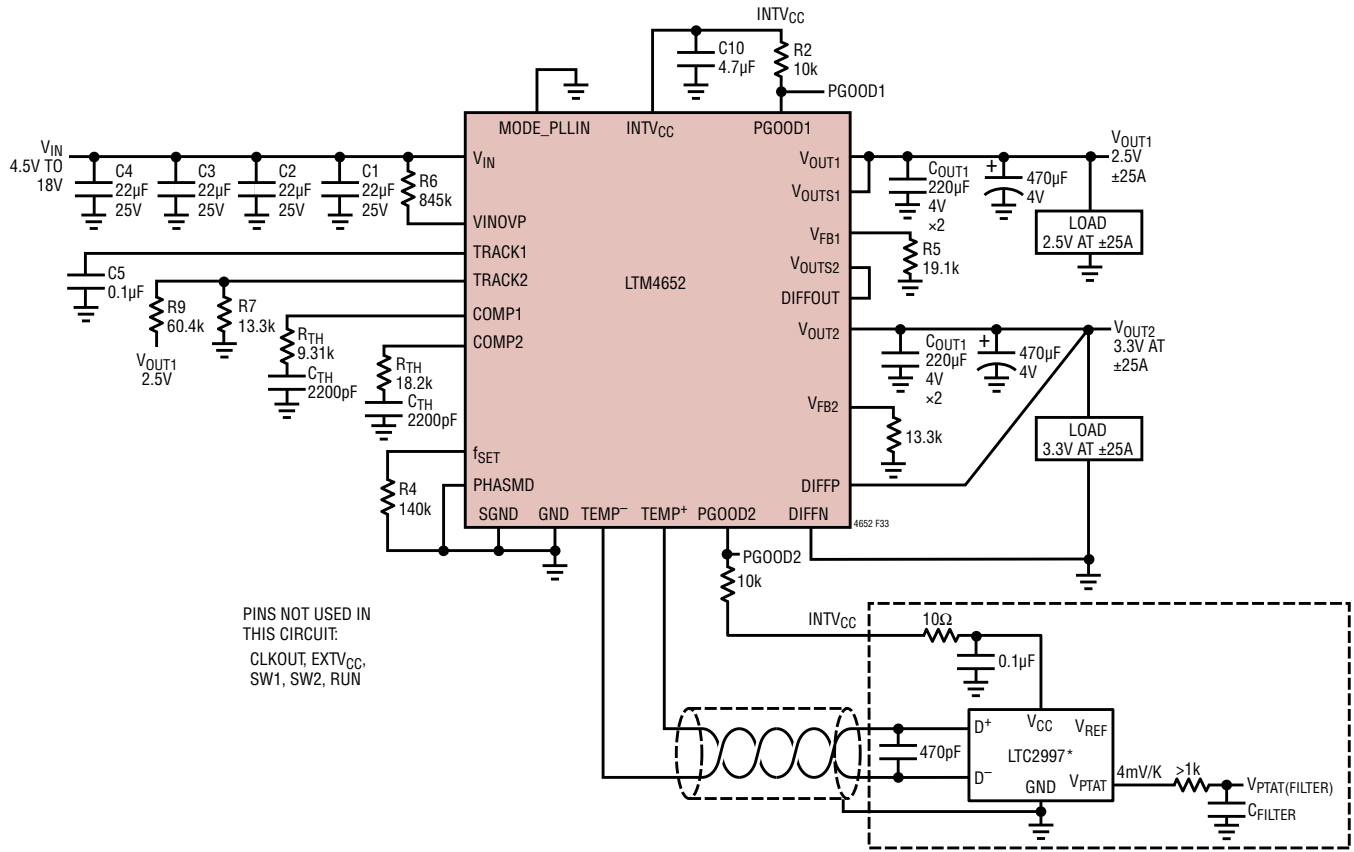
OPTIONAL ANALOG OUTPUT TEMPERATURE INDICATOR
