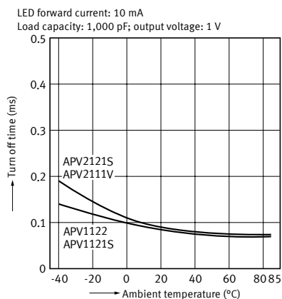
7. Turn off time vs. ambient temperature characteristics
