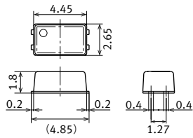
External dimensions
