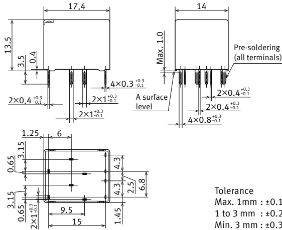
External dimensions
