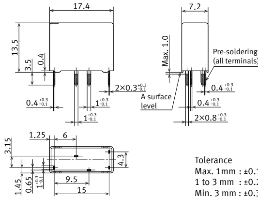
External dimensions
