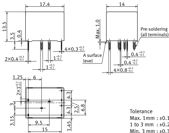
External dimensions
