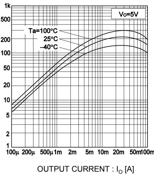
Fig.4 DC current gain vs. output current
